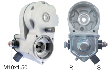
66-82640 Solenoid Switch Assembly 3-Terminals, M12 Battery Post
