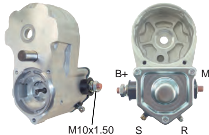
66-82639 Solenoid Switch Assembly 3-Terminals, M10 Battery Post
