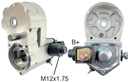
66-82642-1 Solenoid Switch Assembly 3-Terminals, M12 Battery Post
