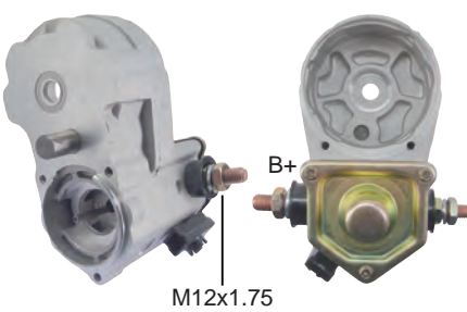
66-82650 Solenoid Switch Assembly 3-Terminals, M12 Battery Post
