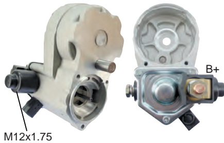
66-82645-1 Solenoid Switch Assembly 3-Terminals, M12 Battery Post
